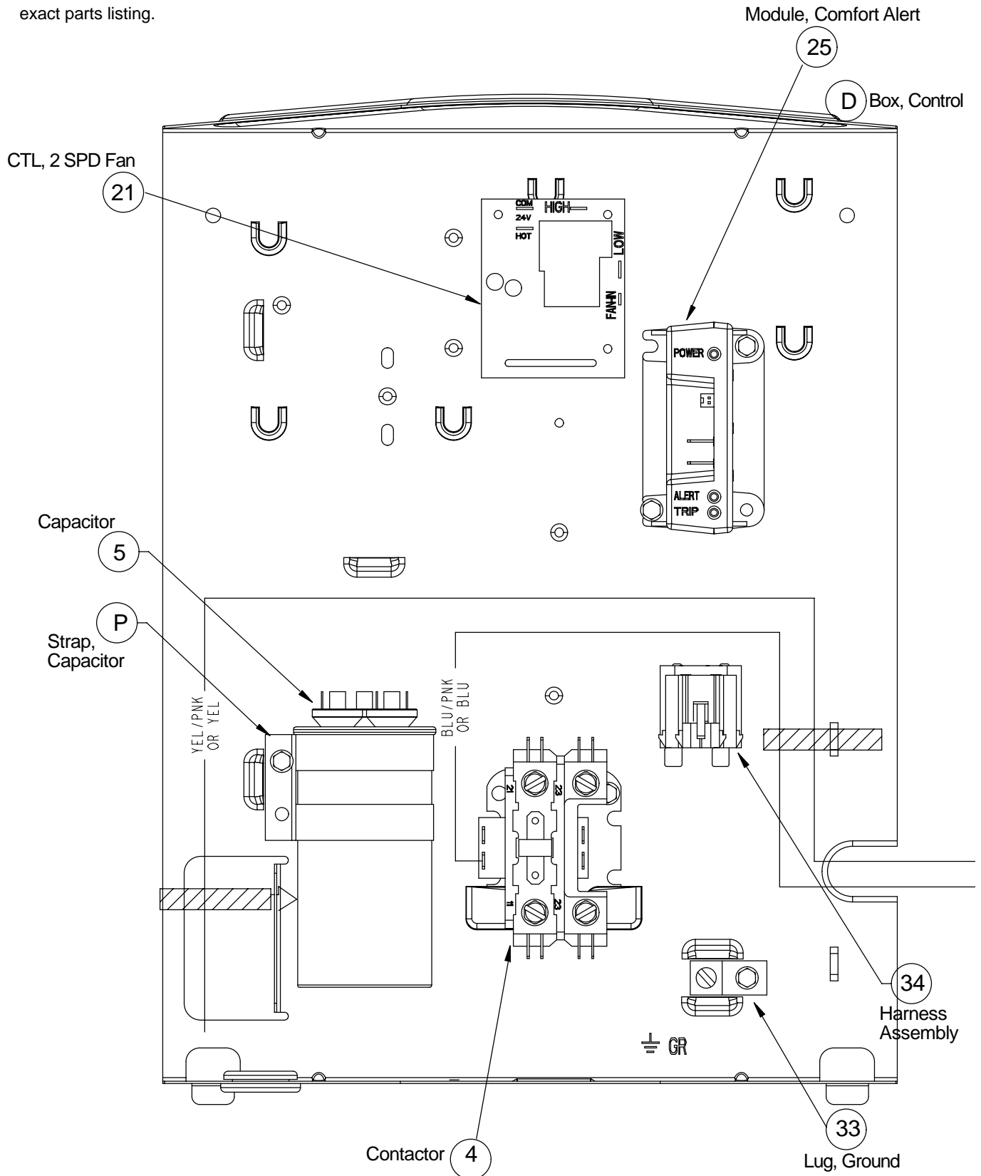
H4A3**GKD100 control box
